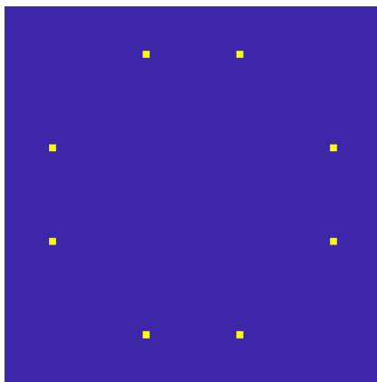
(b) 16-QAM-PCS: c_0 = 1
