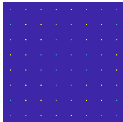
(f) 64-QAM-PCS: c_0 = 1.25
